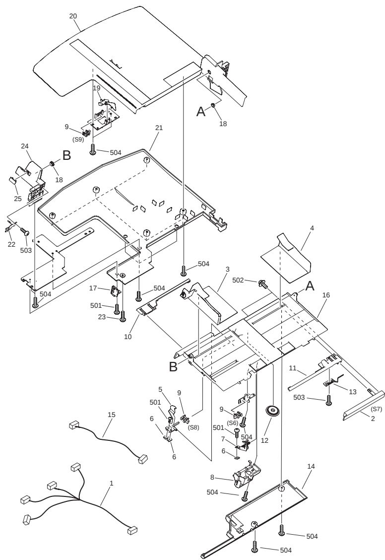
FIGURE P13 PICK-UP TRAY LOWER ASSEMBLY
