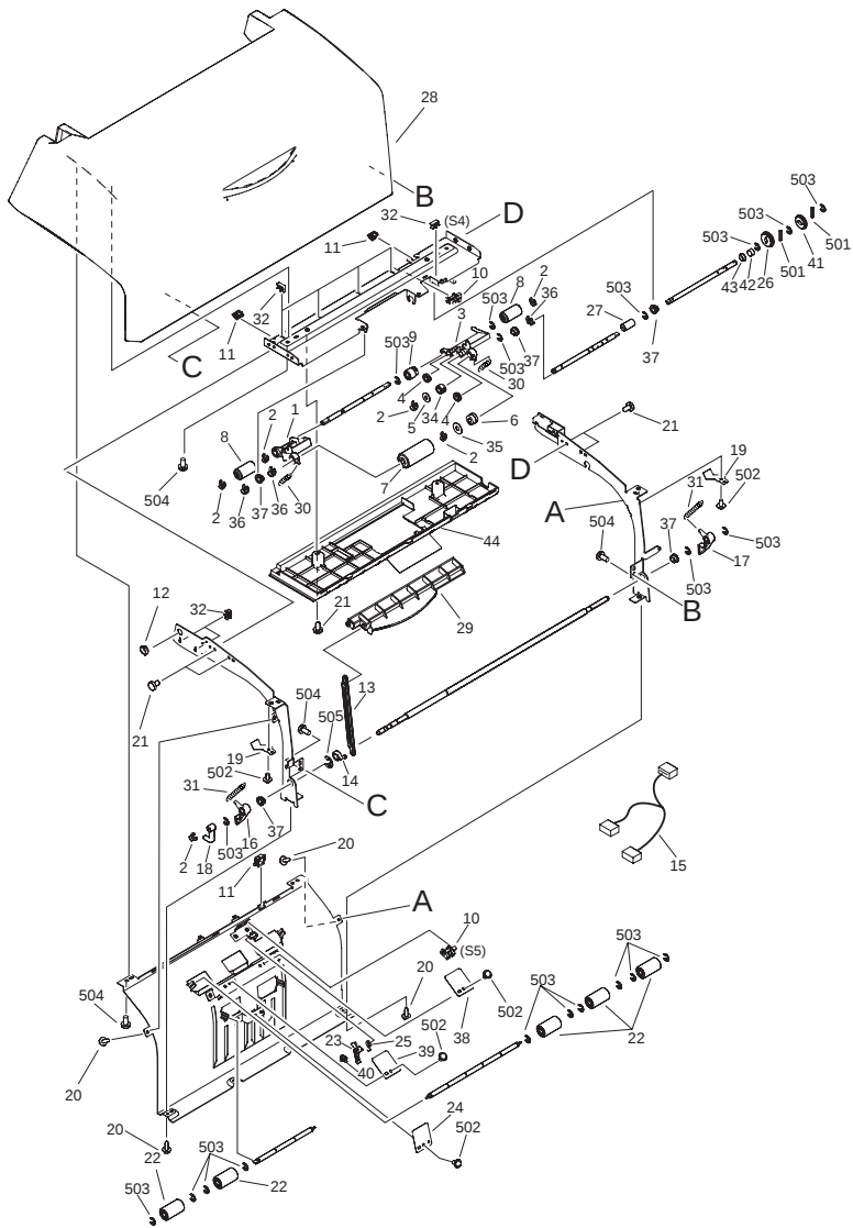
FIGURE P14 UPPER PANEL ASSEMBLY
